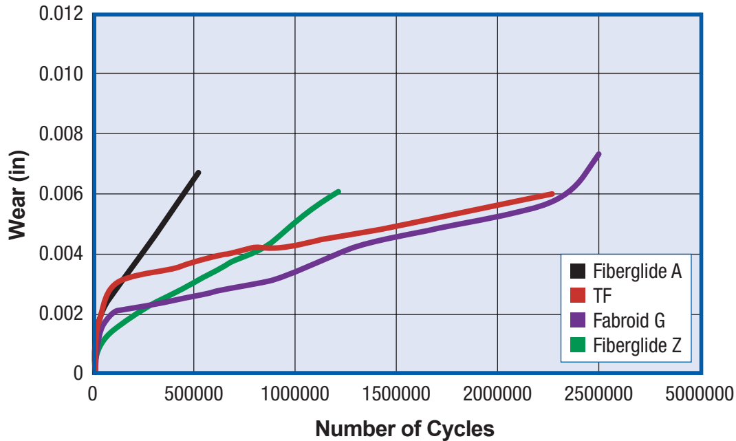
Wear @ 10 ksi
