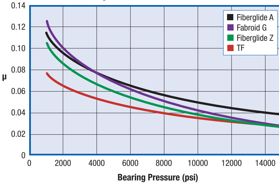
Dynamic Friction vs. Load
